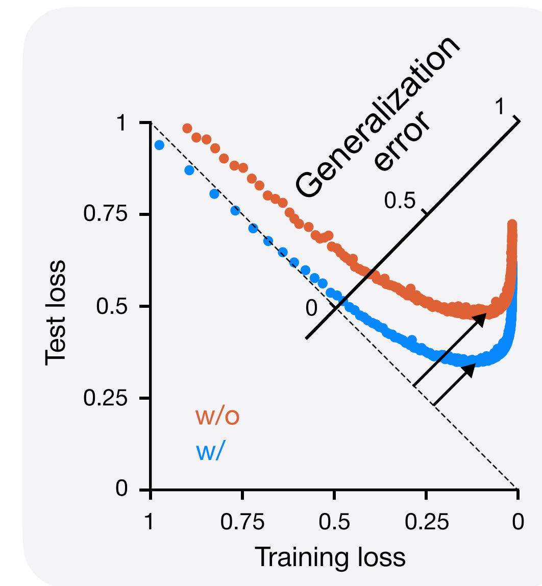
ID generalization
