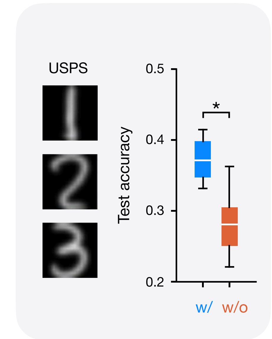
OOD generalization
