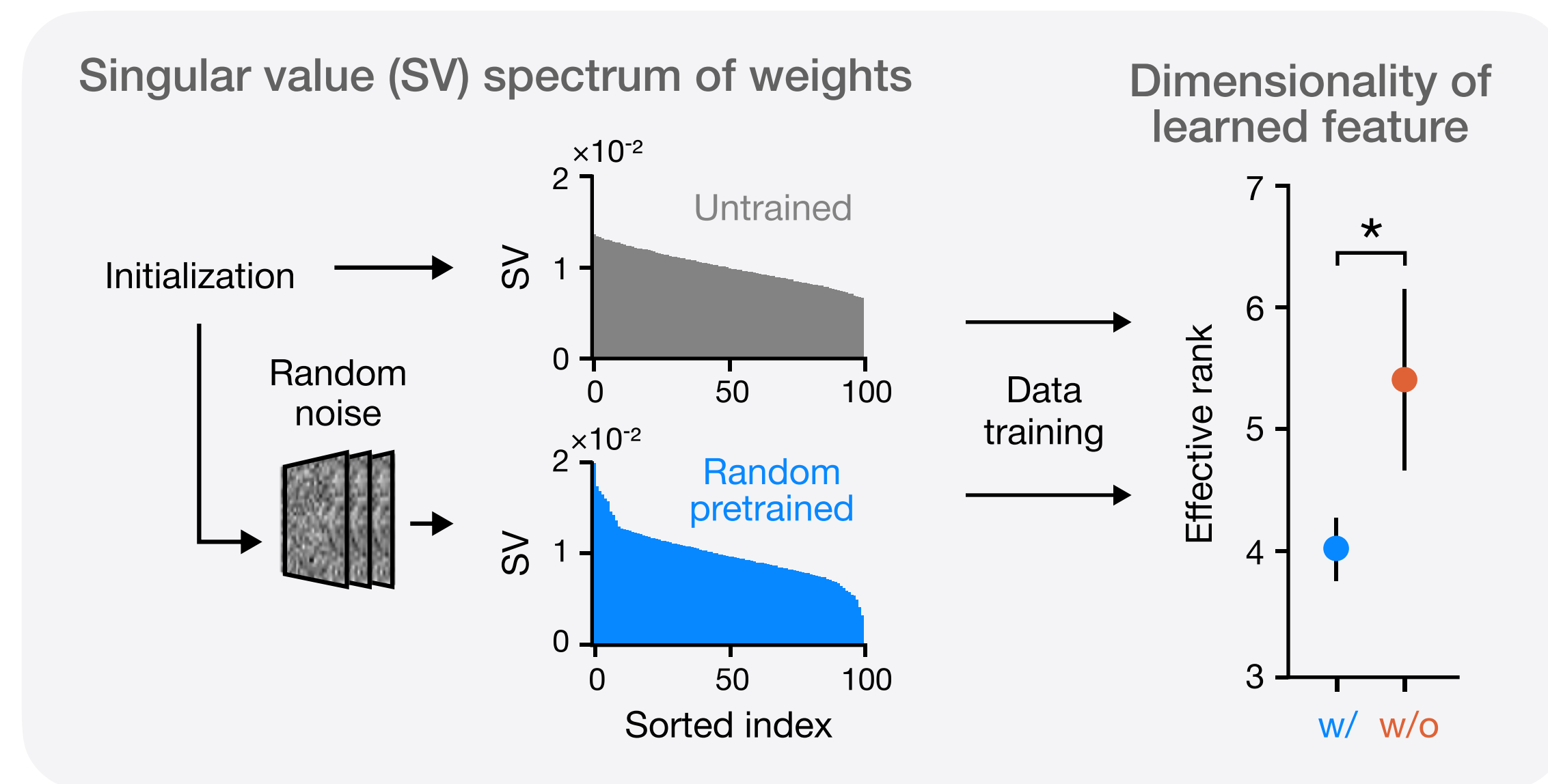
Pre-regularization for learning a low-rank solution
